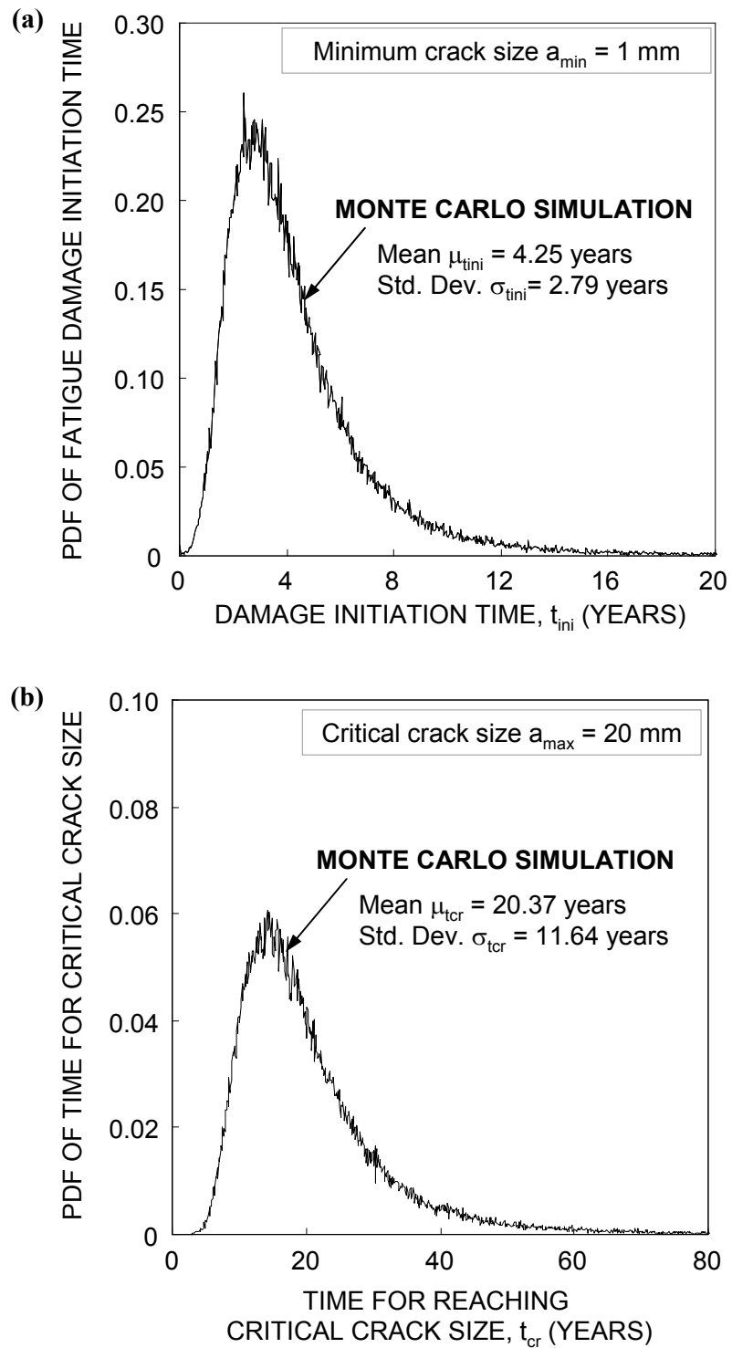
Figure 6.4 PDFs of (a) fatigue damage initiation time; and (b) time to reach the critical crack size
