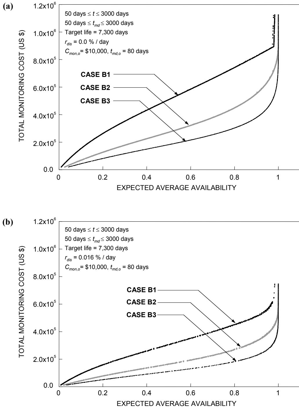
Figure 4.11 Pareto solution sets of multi-objective problem for Case B1, B2 and B3; (a) without discount rate of money; and (b) with discount rate of money r_{dis} = 0.016\% / \text{day}
