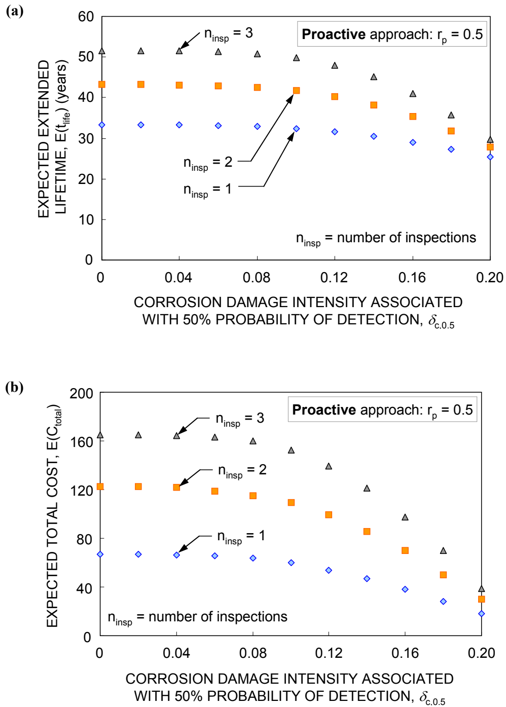
Figure 7.10 Effects of number of inspections on (a) expected extended lifetime; and (b) expected total cost
