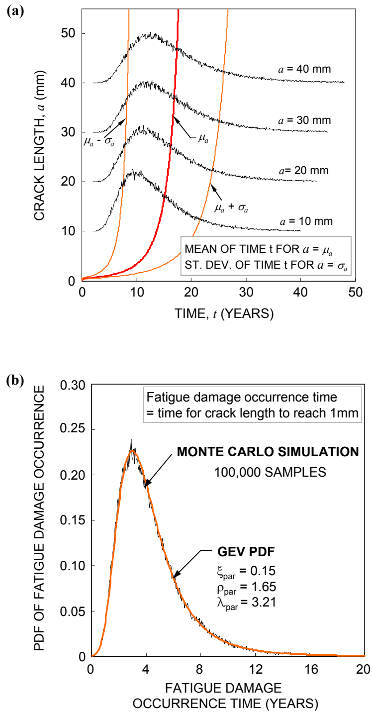
Figure 5.16 (a) Time-variant crack length with PDFs of times when a = 10 mm, 20mm, 30mm, and 40mm; and (b) GEV PDF of fatigue damage occurrence time
